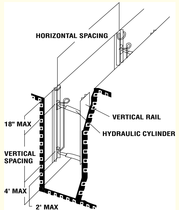
FIGURE D-1 Vertical aluminum hydraulic shoring (spot bracing).
