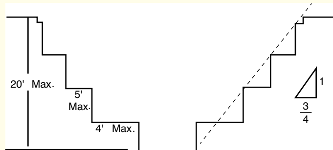
MULTIPLE BENCH
