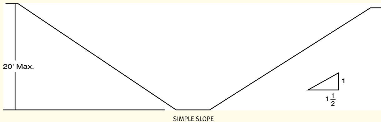
FIGURE B-1-3 Slope Configurations. Excavations Made in Type C Soil. (Continues)
