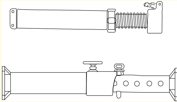
FIGURE E-2 Pneumatic/hydraulic shoring.
