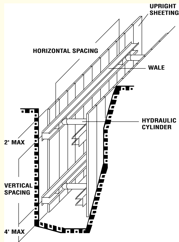
FIGURE D-4 Aluminum hydraulic shoring—Waler System (typical).
