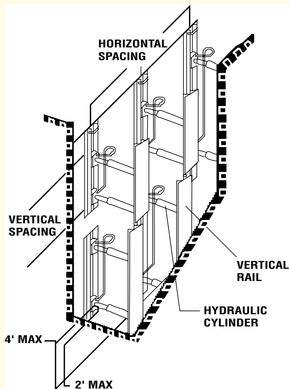
FIGURE D-3 Vertical aluminum hydraulic shoring (stacked).
