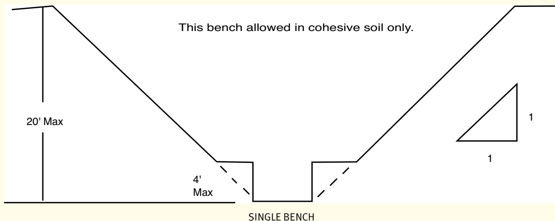
FIGURE B-1-2 Slope Configurations. Excavations Made in Type B Soil. (Continues)
