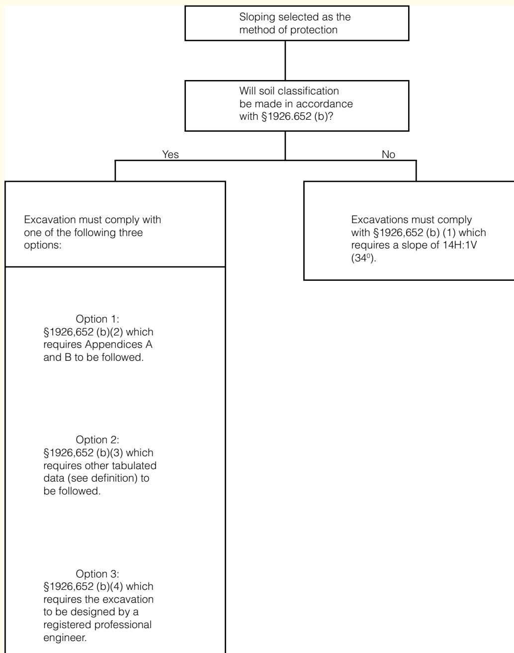
FIGURE F-2 Sloping options.
