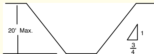
SIMPLE SLOPE—GENERAL
