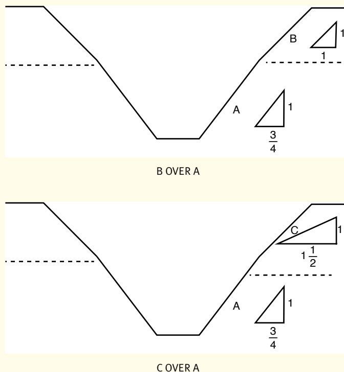
FIGURE B-1-4 Slope Configurations. Excavations Made in Layered Soils. (Continues)
