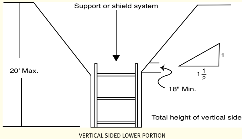
FIGURE B-1-3 Slope Configurations. Excavations Made in Type C Soil. (Continued)
