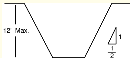
SIMPLE SLOPE—SHORT TERM
