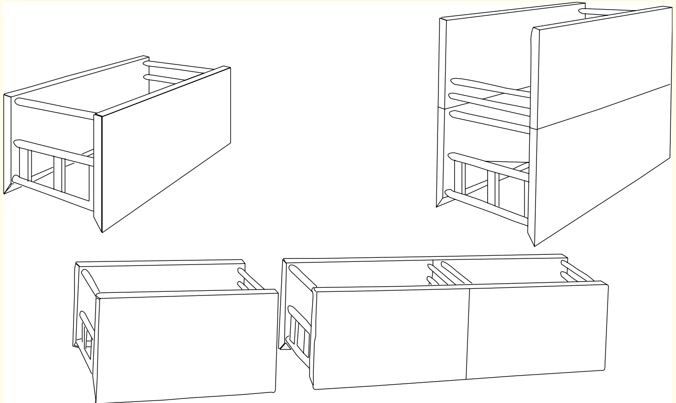
FIGURE E-4 Trench shields.
