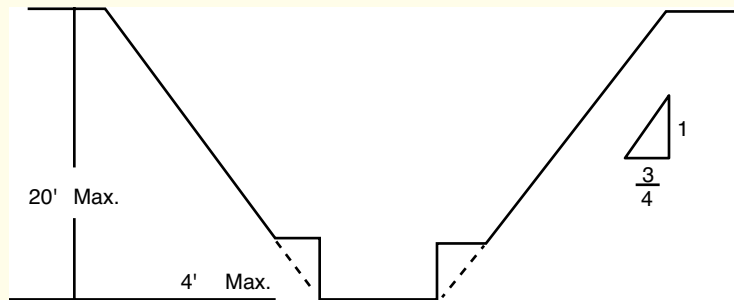
SIMPLE BENCH
