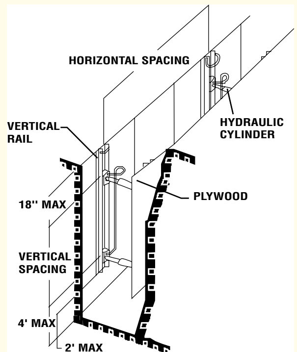
FIGURE D-2 Vertical aluminum hydraulic shoring (with plywood).
