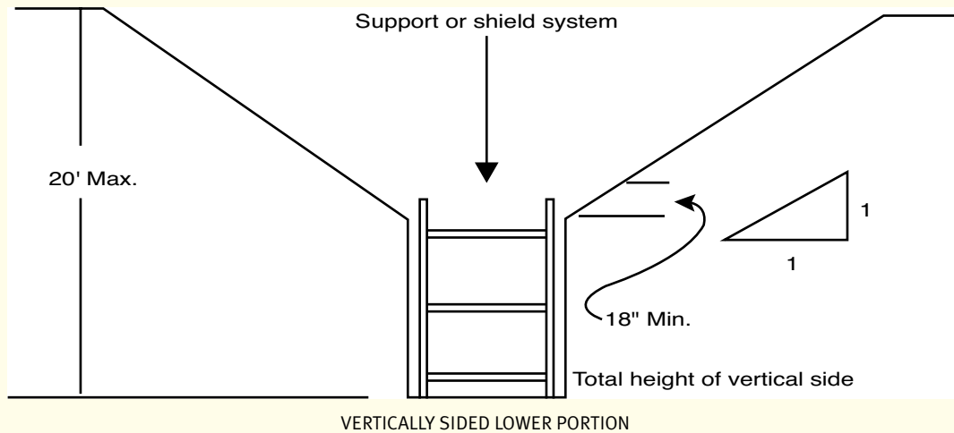
FIGURE B-1-2 Slope Configurations. Excavations Made in Type B Soil. (Continued)
