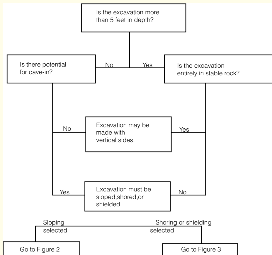
FIGURE F-1 Preliminary decisions.
