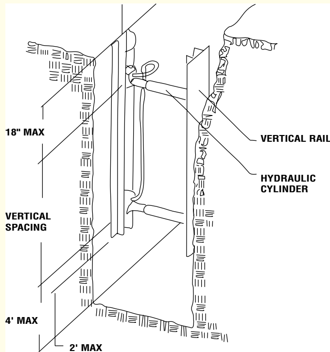
FIGURE E-1 Aluminum hydraulic shoring.
